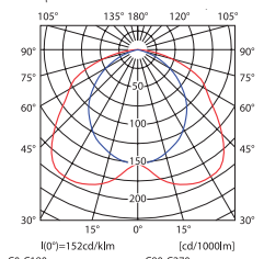
OFRA TL-236B CO-C180 \eta(0^\circ)=152\text{cd/klm} C90-C270 [cd/1000lm]
