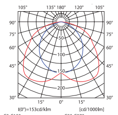
OFRA TL-218B CO-C180 \eta(0^\circ)=153\text{cd/klm} C90-C270 [cd/1000lm]
